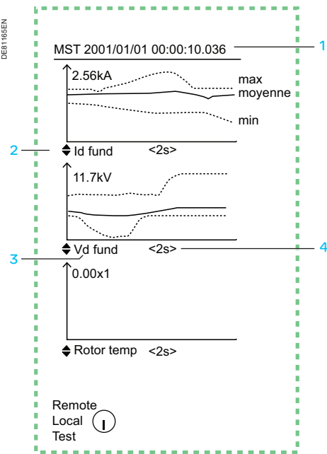
Visualisation of 3 graphics MST via an integrated synoptic HMI.
